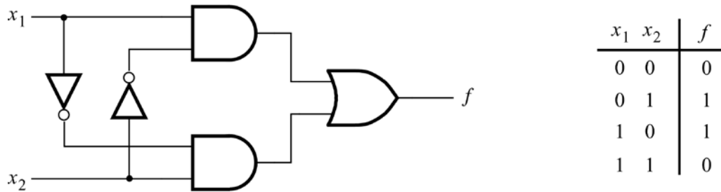
Figure 12. The light controller circuit.
